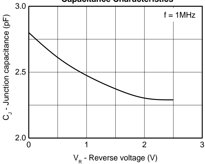
Capacitance Characteristics
