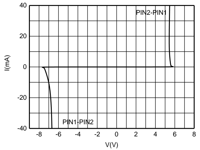
I-V Curve
