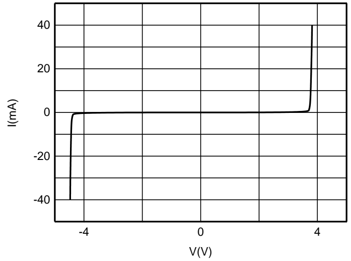
I-V Curve
