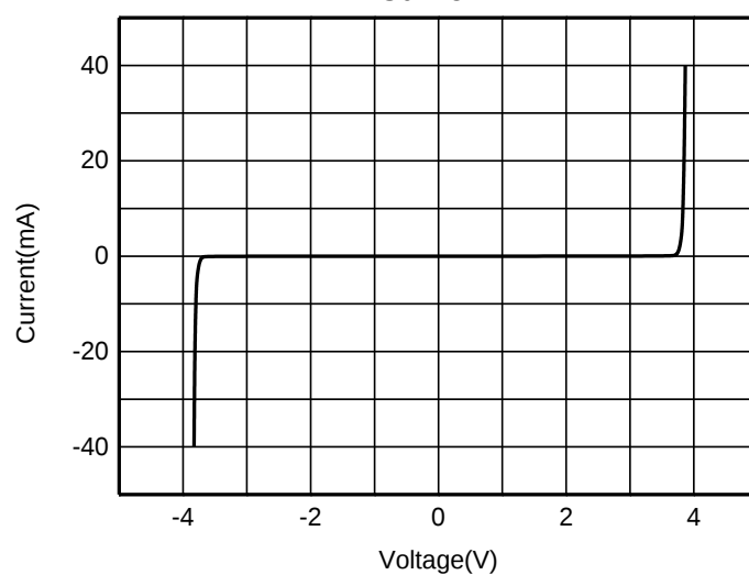
I-V Curve
