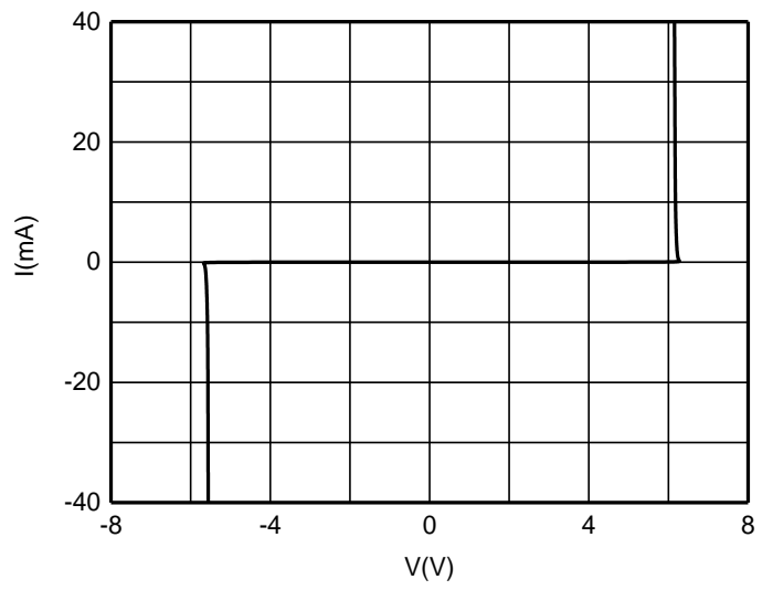
I-V Curve
