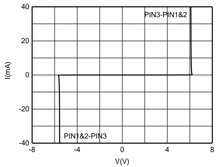
I-V Curve
