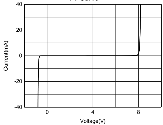
I-V Curve
