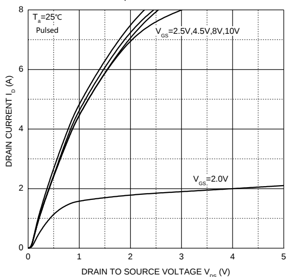
Output Characteristics
