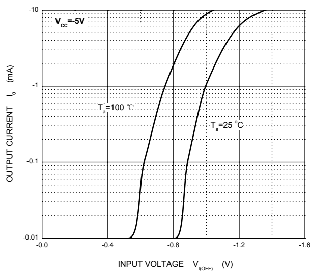
OFF Characteristics
