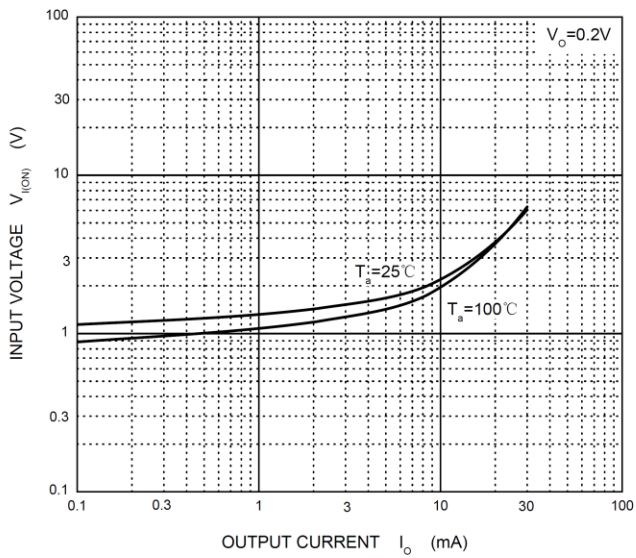
ON Characteristics
