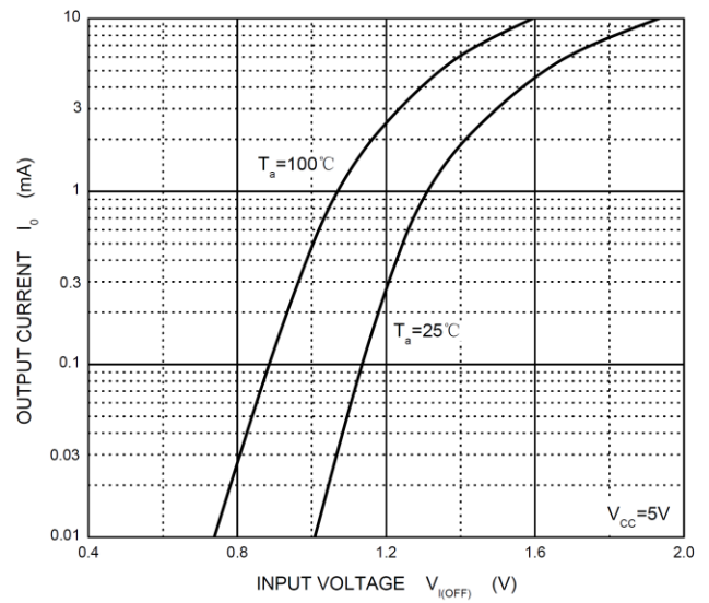
OFF Characteristics
