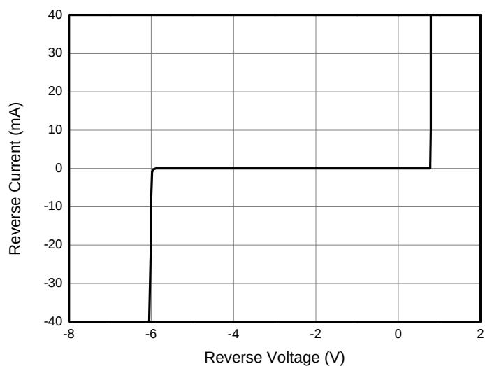
I-V Curve
