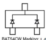
BAT54CW Marking: L43
