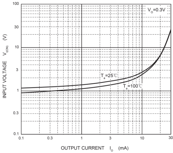
ON Characteristics
