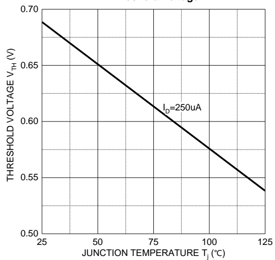
Threshold Voltage
