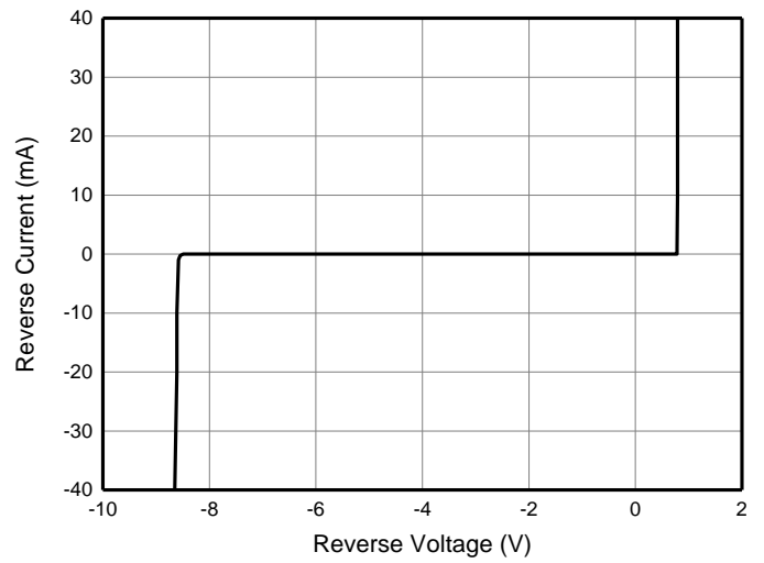
I-V Curve
