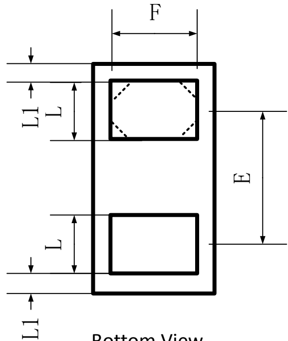
Bottom View
