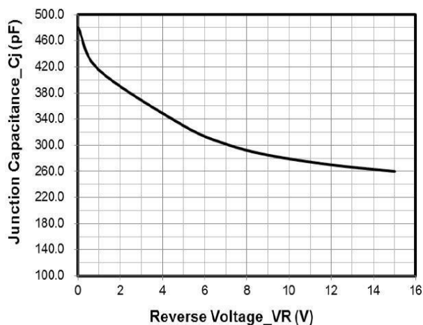
Novction Capacitance vs. Reverse Voltage
