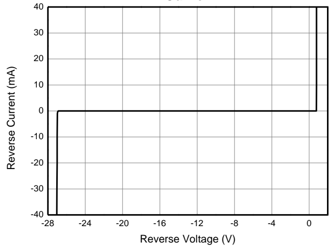
I-V Curve
