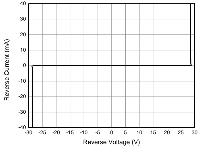
I-V Curve
