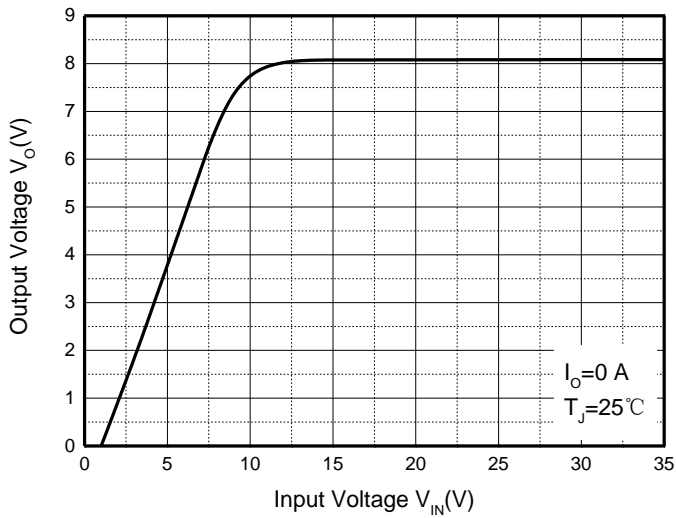
Output Characteristics
